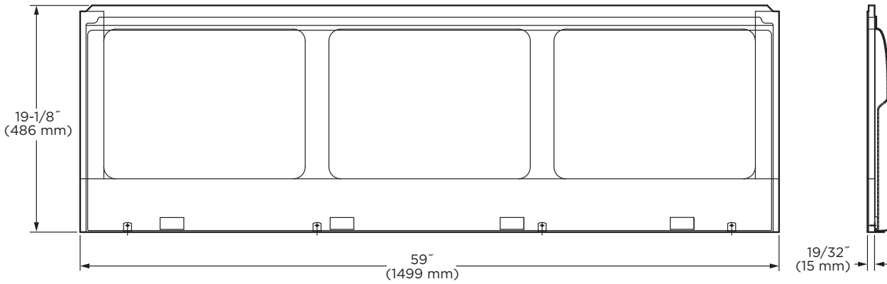
4813-00 60" (1524 mm) Apron for Stratton
